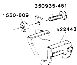
522443 FINGER GUARD (NOT OPERATOR REMOVABLE) FOR DOMESTIC AND EXPORT
